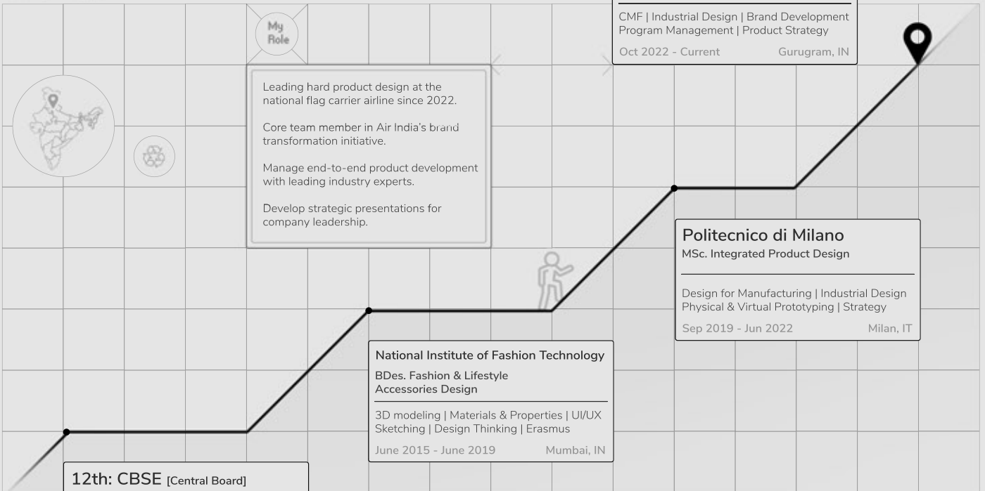
Fig 0.1 - Journey Graph
